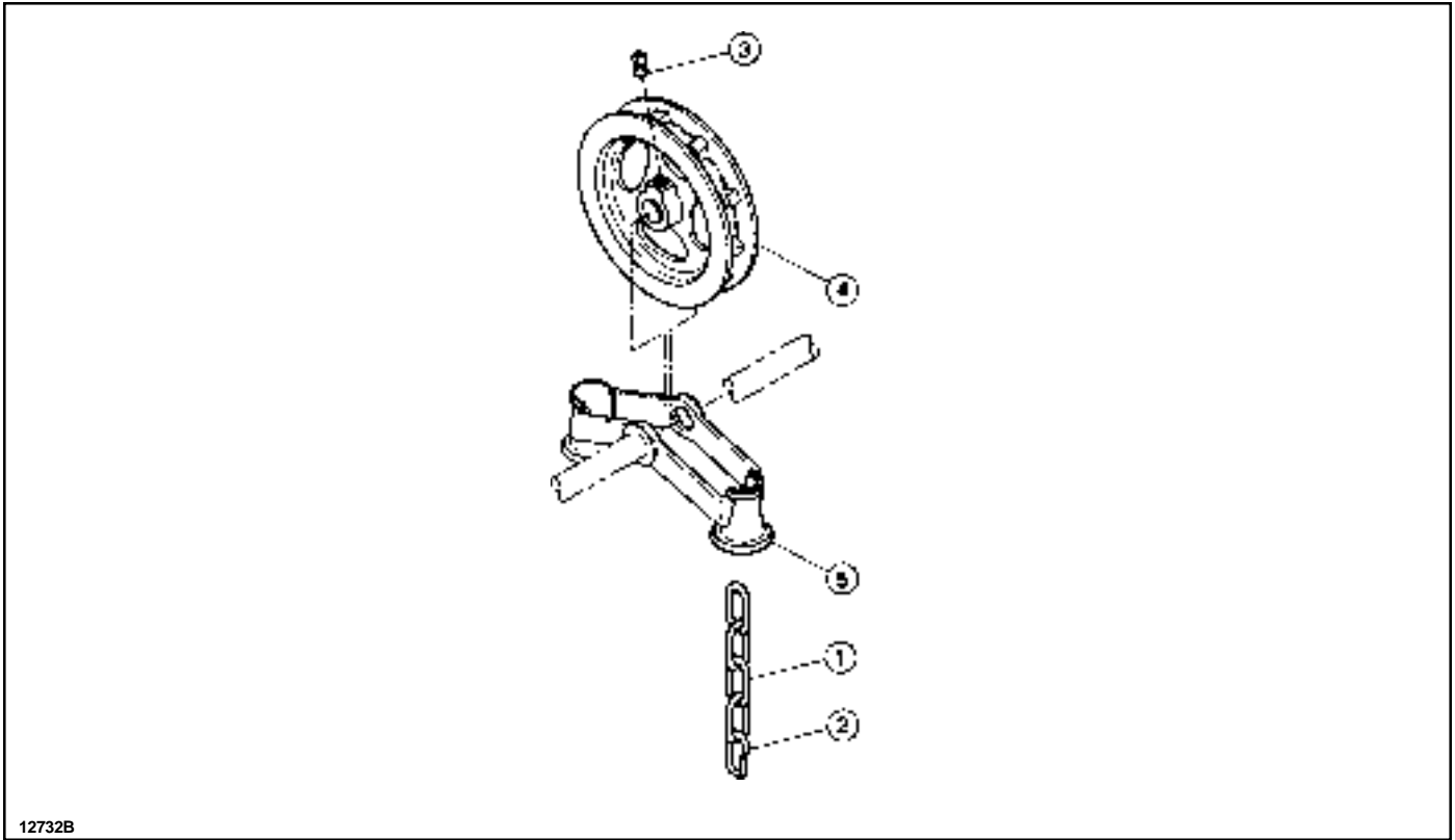
Figure 4. Hand Chain Drive. (Catalog Numbers 8282 and 913115).
