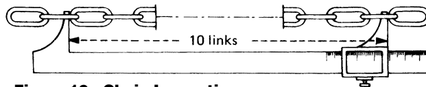
Figure 10 - Chain Inspection
